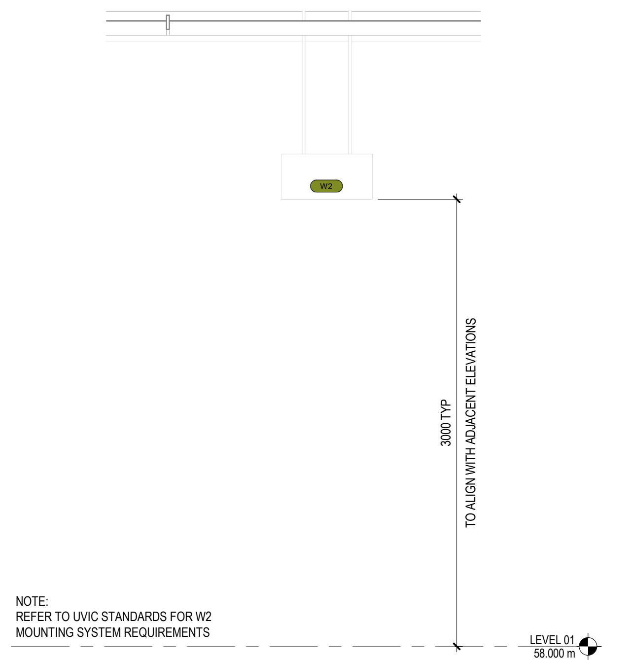
4 SUSPENDED SIGNAGE- AT CEILINGS OVER 3m 1:25
