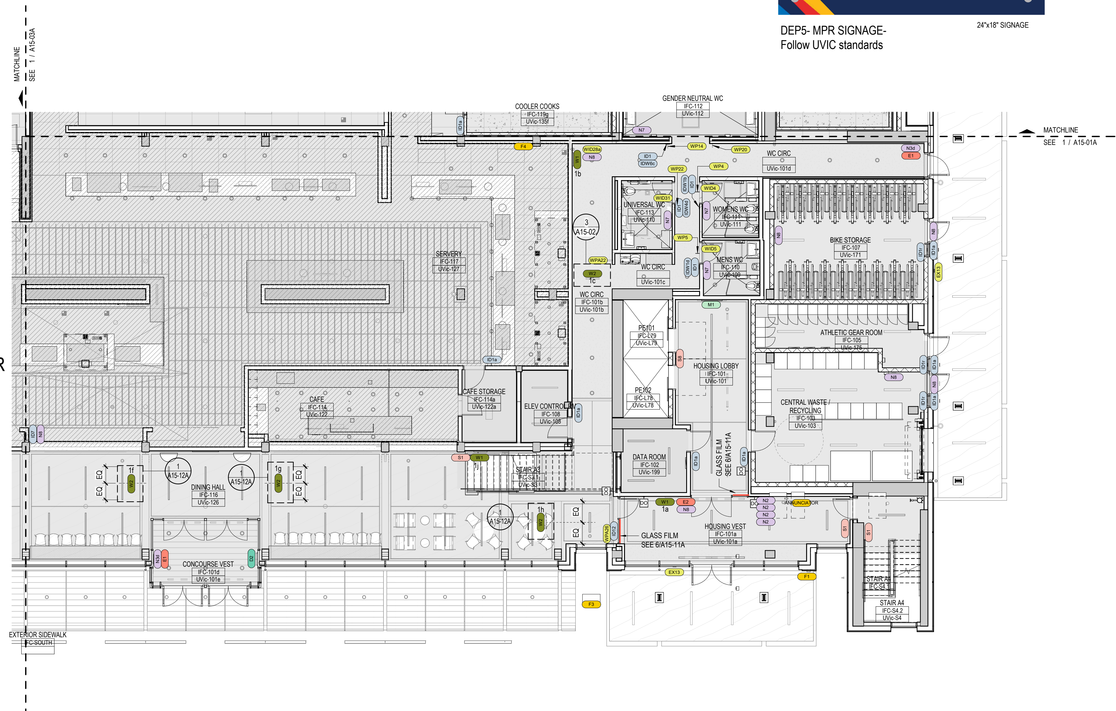
1 SIGNAGE PLAN L01-SE 1:100
